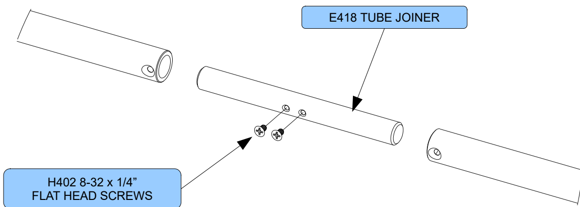
E418 tube joiner bar assembly
