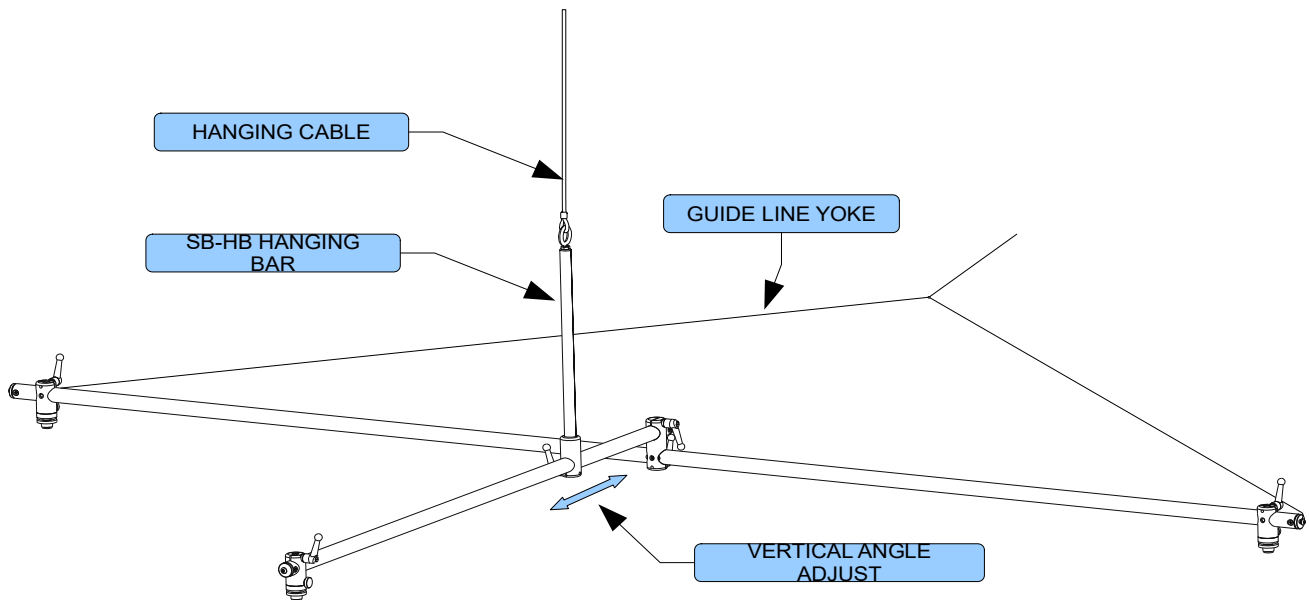
Decca Tree with SB-HB Hanging Bar
